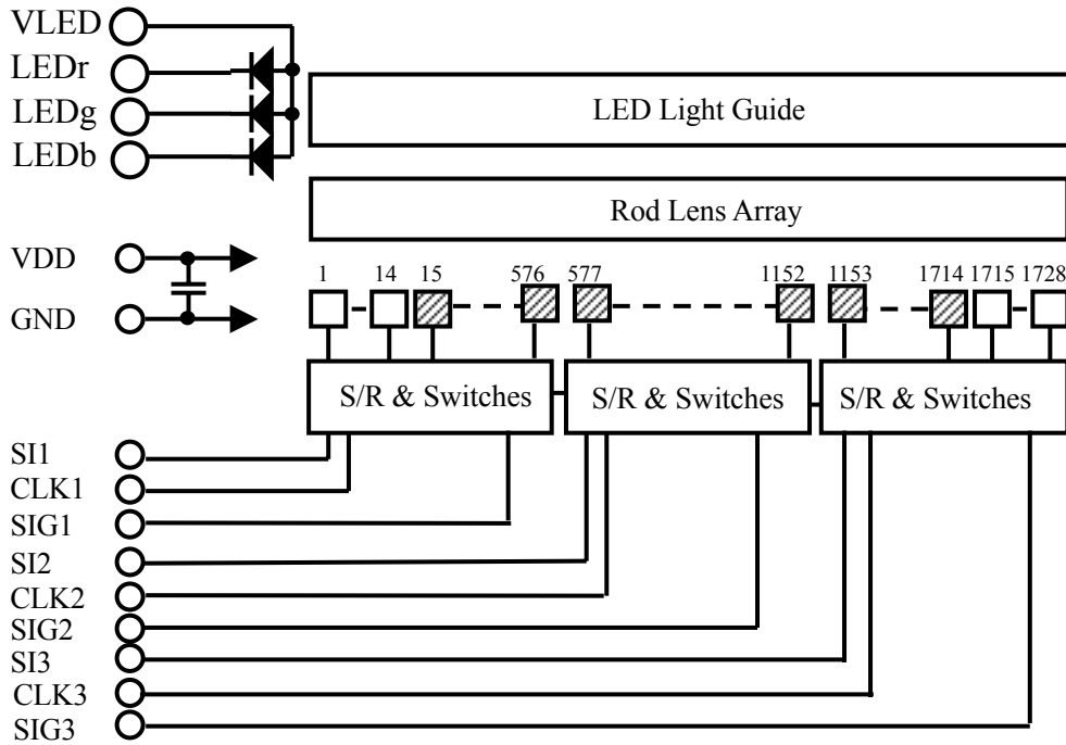
Figure 5. Block Diagram
