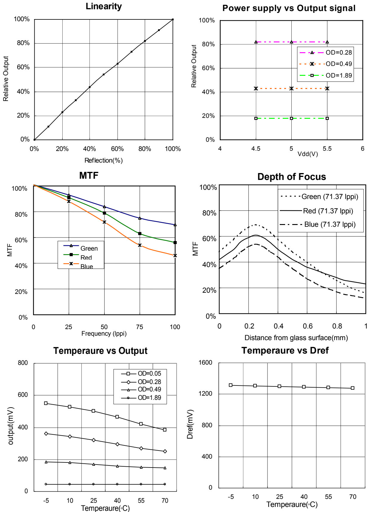
Figure 13. Typical Performance Curve Unless otherwise specified, T_a=25^\circ
