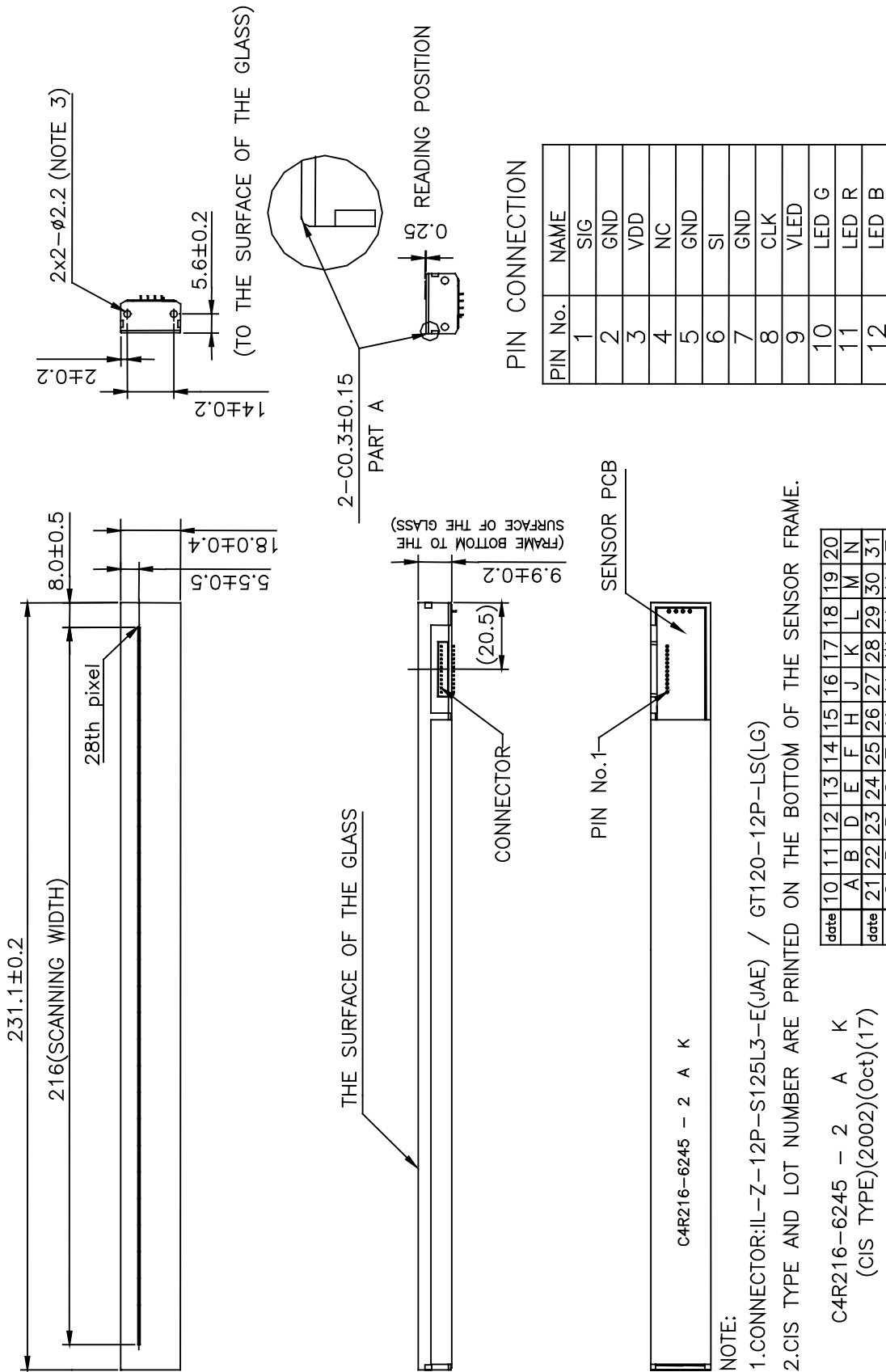
Figure 1 Dimensions
