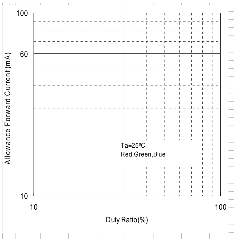
Figure 3. Duty Ratio vs Allowable Forward Current
