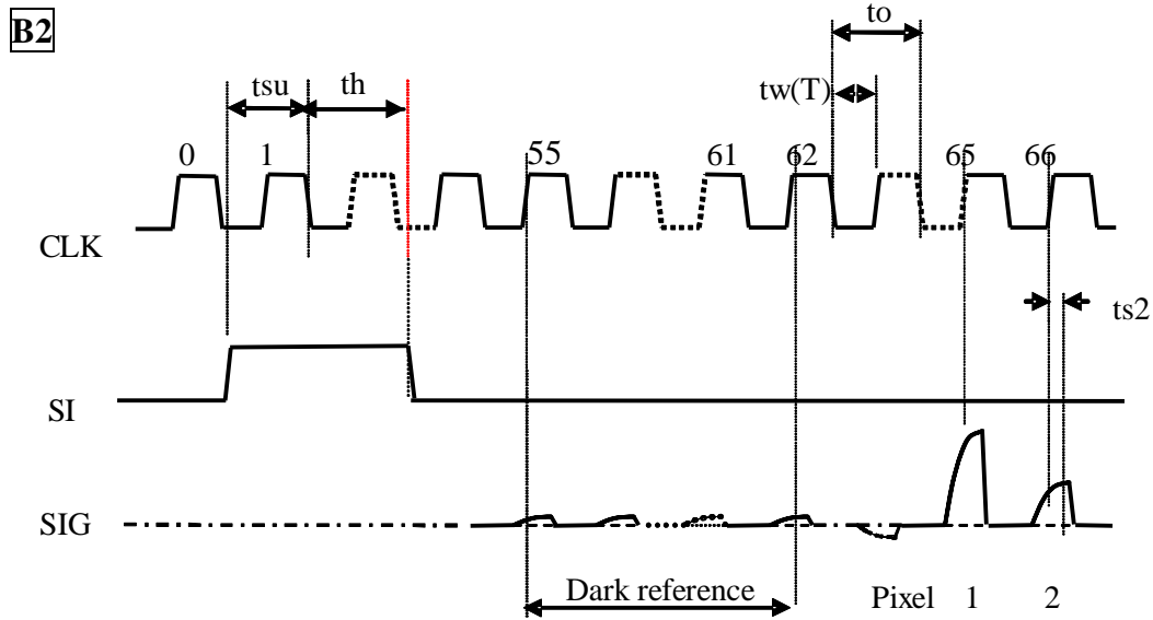
Figure 4 Timing Diagram
