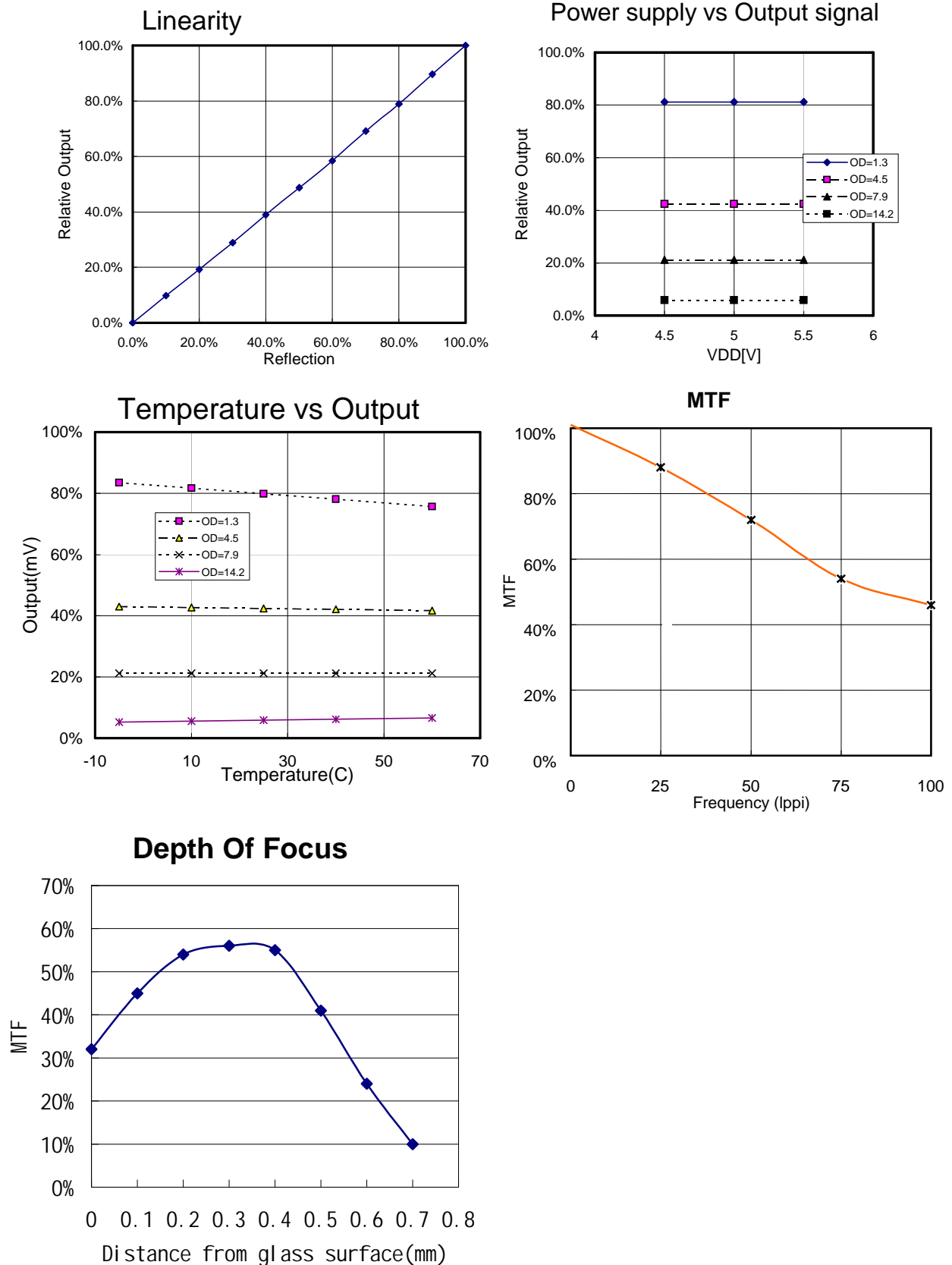
Figure 8. Typical Performance Curve Unless otherwise specified, Ta=25°C
