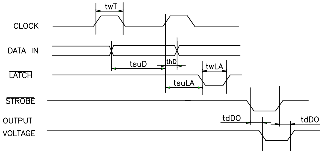
Fig. 2 Thermal Print Head (TX104) Timing Chart
