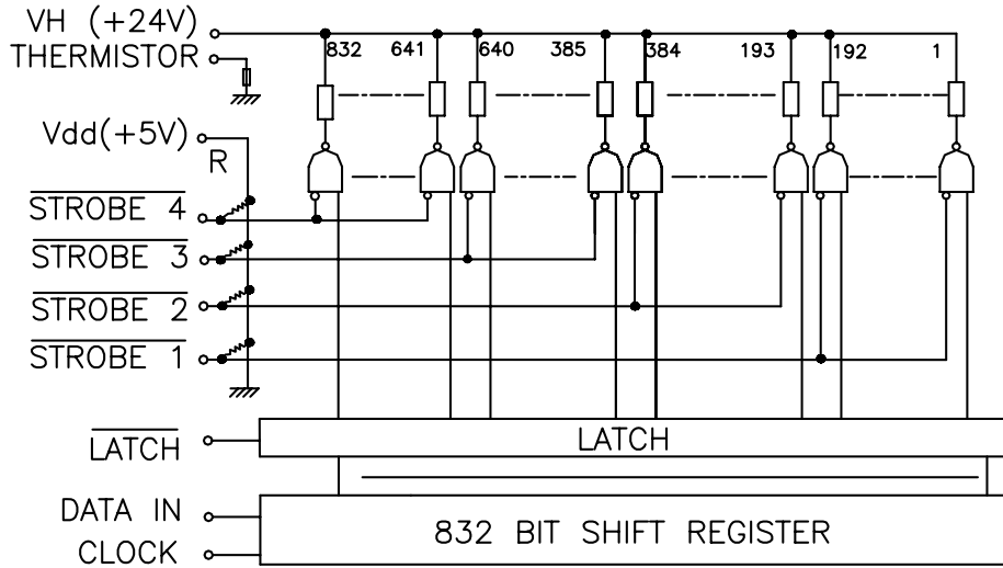
Fig. 3 Schematic Diagram
