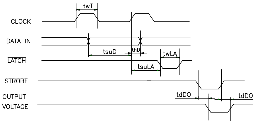
Fig. 2 Thermal Print Head (T80) Timing Chart
