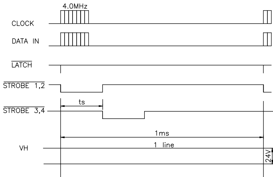
Fig. 2 Thermal Print Head (3J98) Timing Chart
