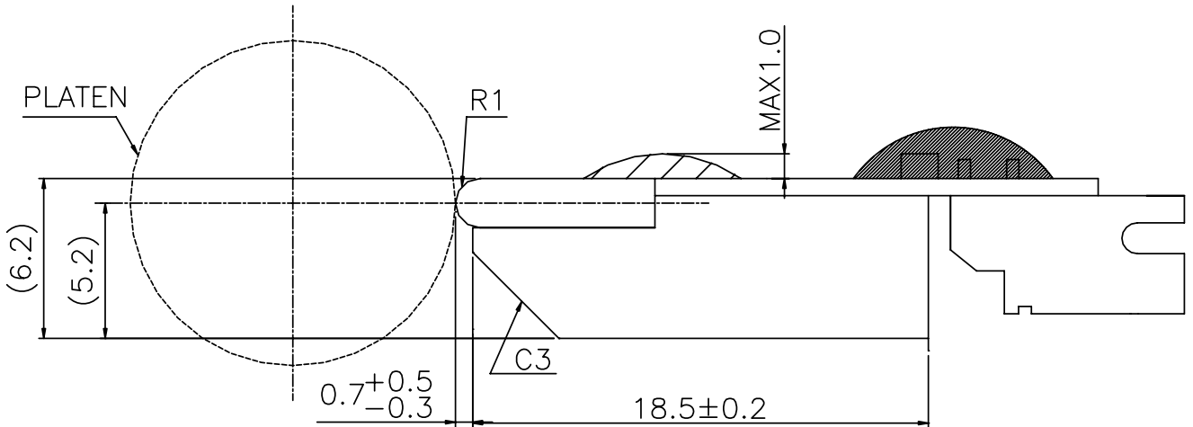
Fig. 4 Cross Section
