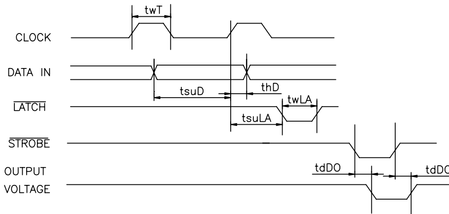
Fig. 2 Thermal Print Head (3J98) Timing Chart
