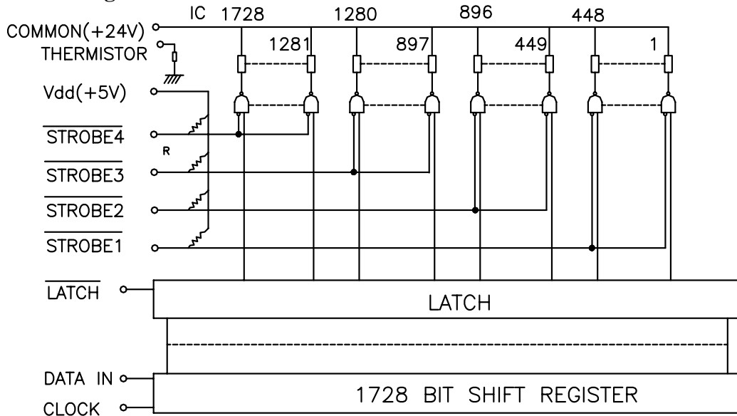
Fig. 3 Schematic Diagram
