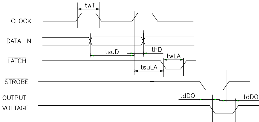
Fig. 2 Thermal Print Head (CH216) Timing Chart
