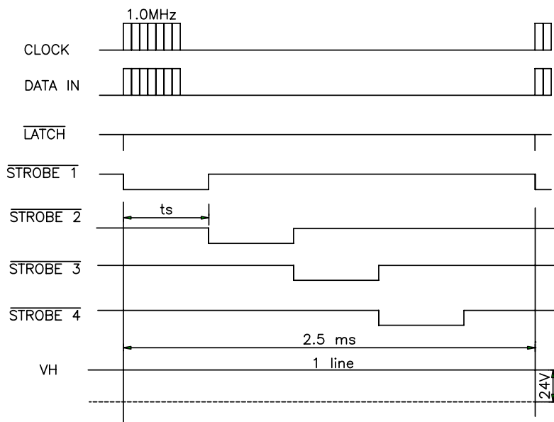
Fig. 2 Thermal Print Head (CH216) Timing Chart
