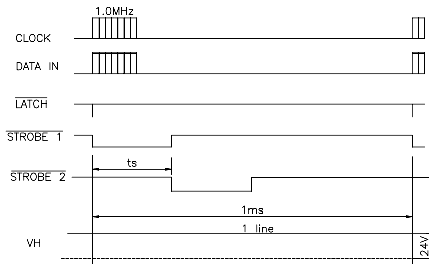
Fig. 2 Thermal Print Head (J32-9774) Timing Chart
