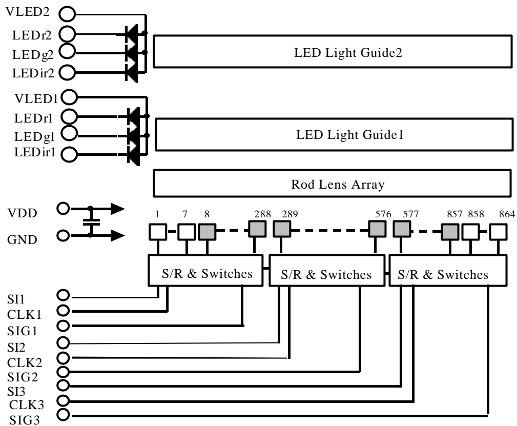
Figure 5. Block Diagram
