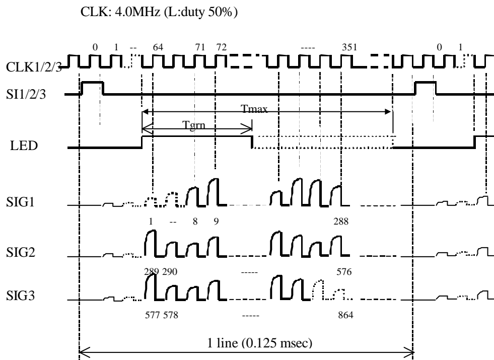
Figure 6. Timing Diagram
